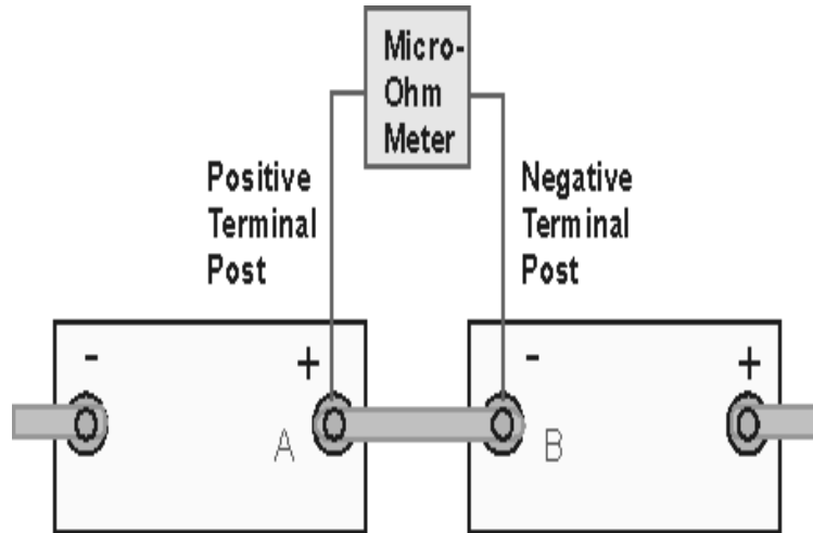
Figure D.4—Single intercell connection
